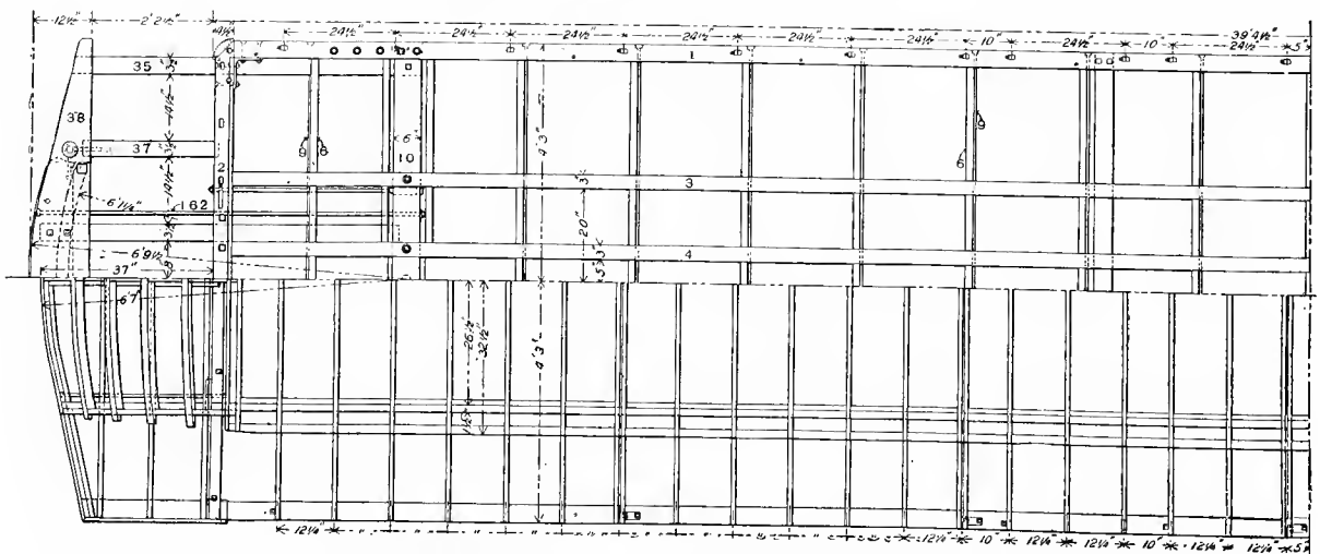
Fig. 463. Half Plan of Underframing and Roof Framing.
